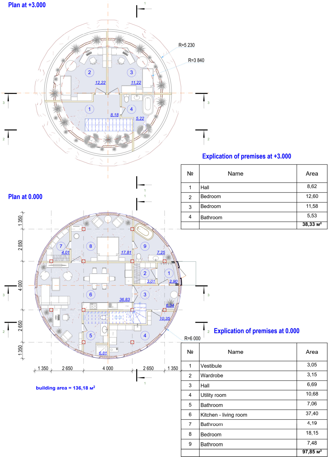
Fig. 1. Floor plans
