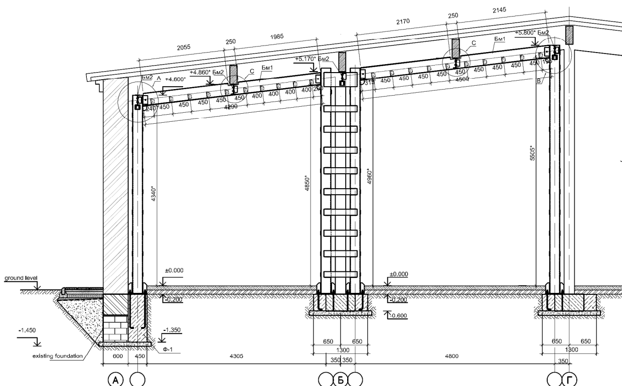
Fig. 7. Cross-section
